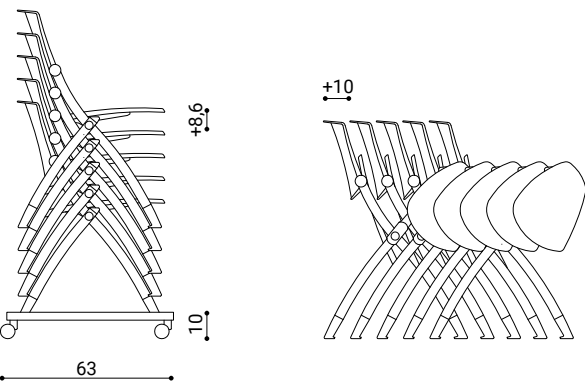
TROLLEY & STORAGE
