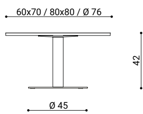
COFFEE TABLE
