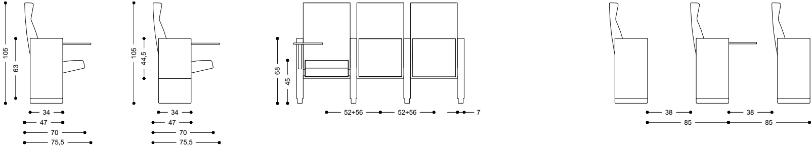
C100 schienale alto - C100 with high backrest
