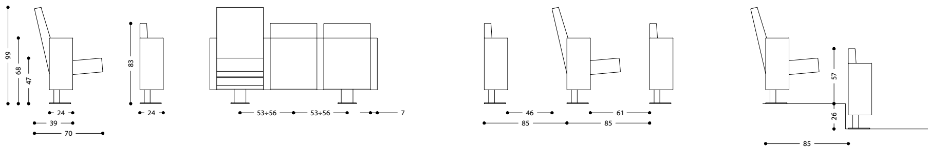
Mura “A”Vip su barra con piede centrale - Mura “A”Vip on beam with central base
