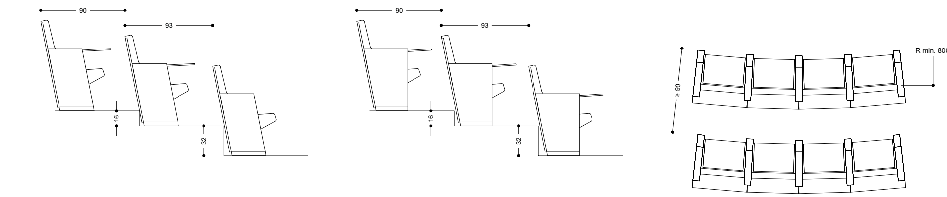
L213 Fiancata standard e maggiorata inclinata o dritta - L213 with standard and increased width side (inclined or straight)
