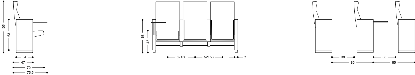
C100 su barra schienale alto - C100 on beam with high backrest
